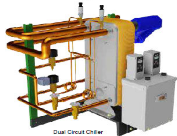
Dual Circuit Chiller
