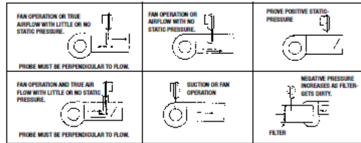
Location of Sample Lines for Typical Applications
